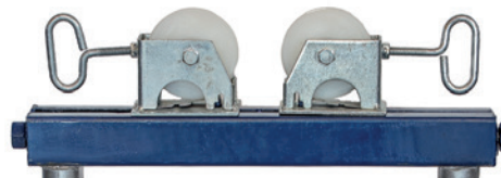
Nylon wheel head NWH 200/501
